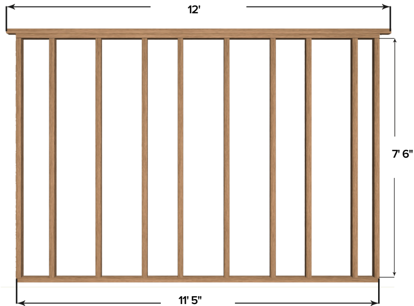
BACK WALL
