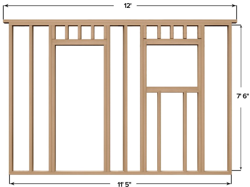
FRONT WALL
