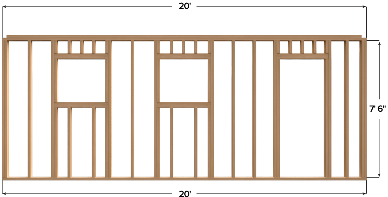
RIGHT WALL
