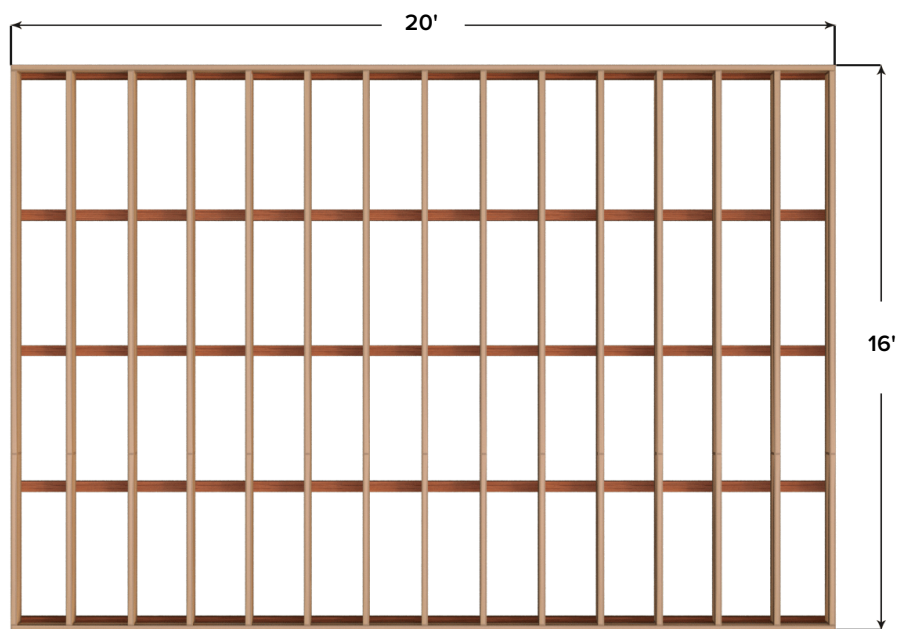
FOUNDATION BASE
